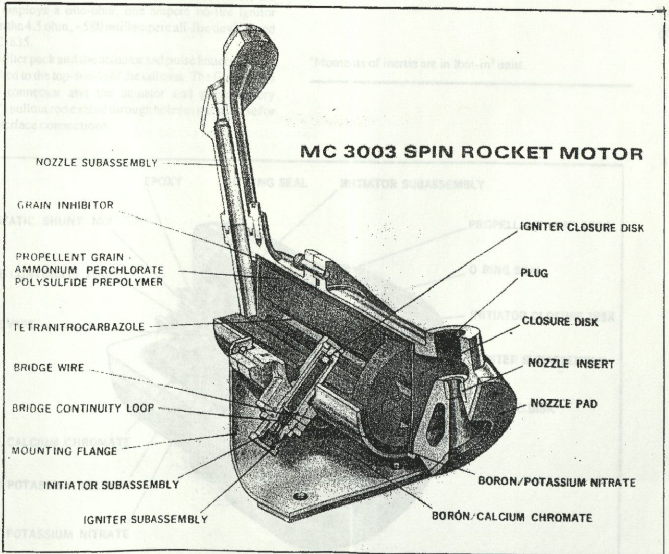
Figure 4 MC3003 Rocket Motor
